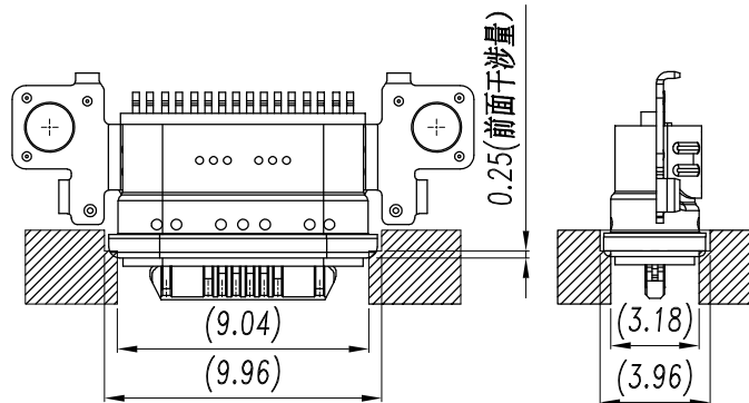
RECOMMENDED CAVITY SIZE
