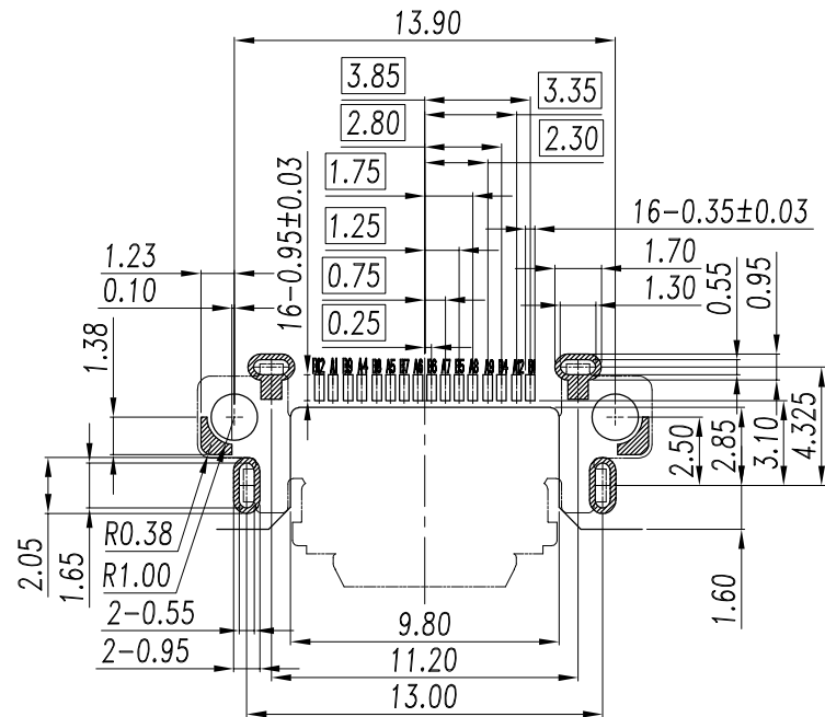
RECOMMENED PCB LAYOUT(T=0.70) SCALE 1:1(GENERAL TOLERANCE±0.05)
