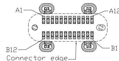
P.C.B LAYOUT VIEW TOLERANCE ±0.05
