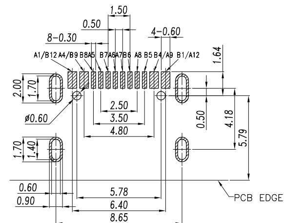
RECOMMENDED P.C.B LAYOUT (COMPONENT SIDE) TOLERANCE FOR PCB LAYOUT IS ±0.05
