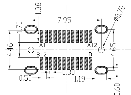
P.C.B LAYOUT VIEW
