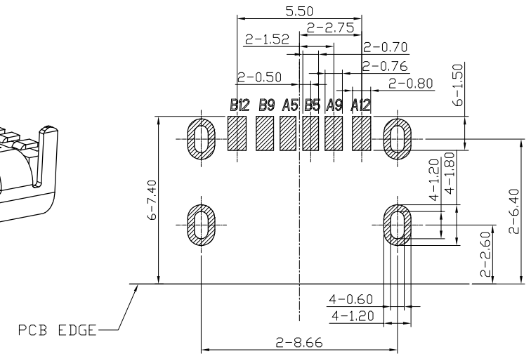
P.C.B LAYOUT VIEW
