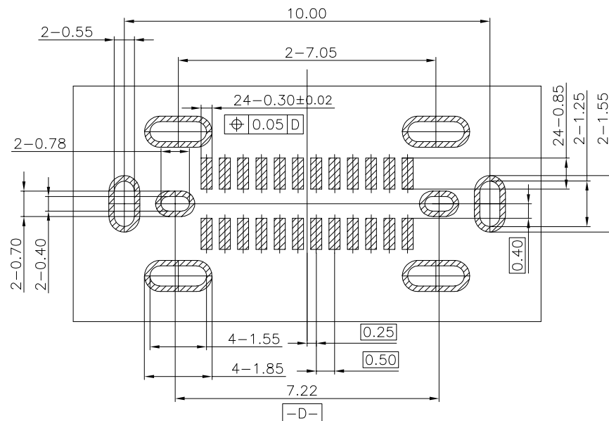
RECOMMENDED PCB LAYOUT (SCALE 2:1) TOLERANCE UNSPECIFIED \pm 0.05\text{mm}
