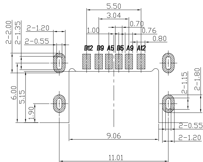
P.C.B LAYOUT VIEW
