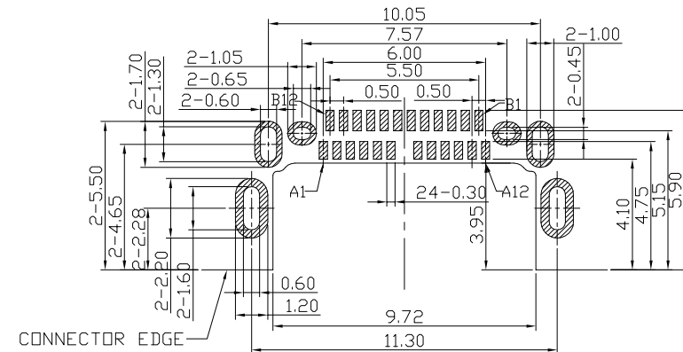
P.C.B LAYOUT VIEW (TOLERANCE ±0.05)
