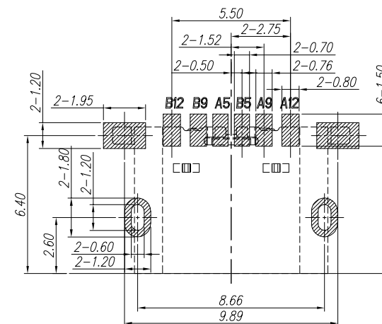
P.C.B LAYOUT VIEW TOLERANCE ±0.05
