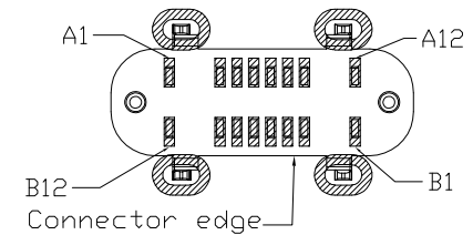
P.C.B LAYOUT VIEW TOLERANCE ±0.05
