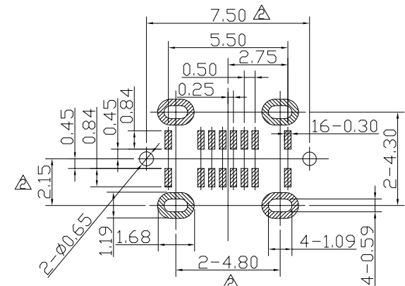
P.C.B LAYOUT VIEW TOLERANCE ±0.05
