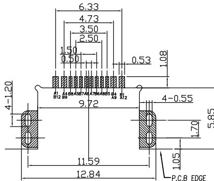
RECOMMENDED PCB LAYOUT(TOP VIEW) DEFAULT TOLERANCE: ±0.05
